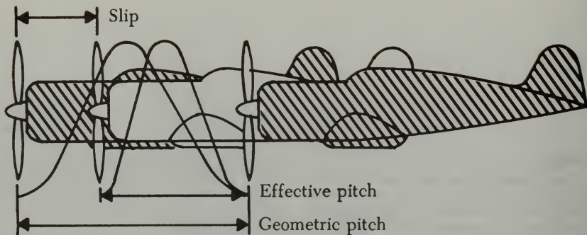
FIGURE 7-1. Effective and geometric pitch.
